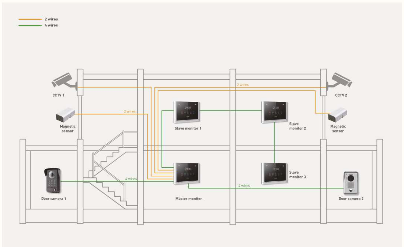
FIELD OF HOME BLACK BOX APPLICATION (4:4:4 AHD SYSTEM)
