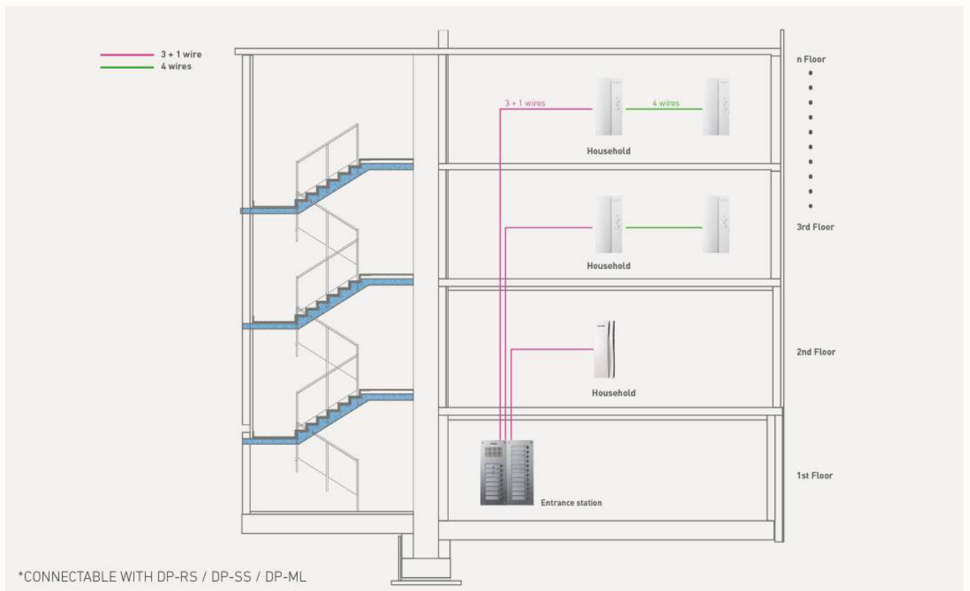
FIELD OF MULTI BUTTON AUDIO UNIT APPLICATION
