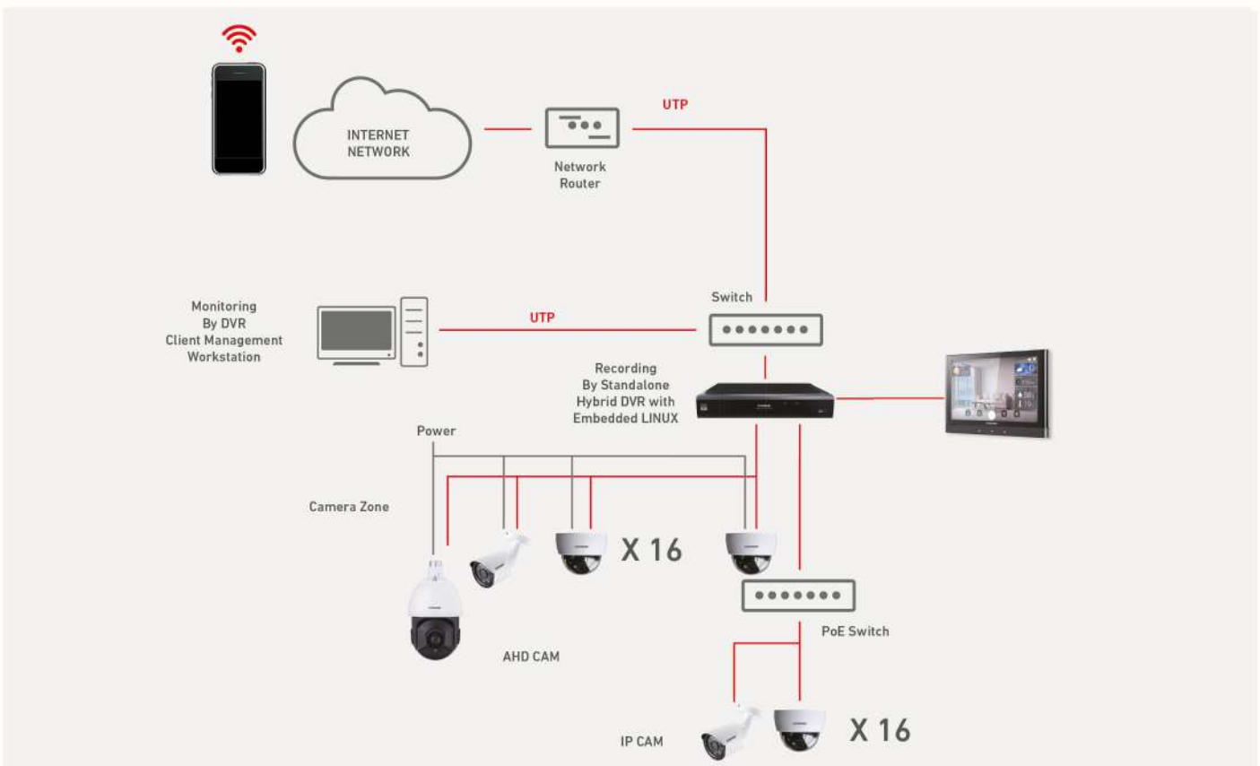
FIELD OF AHD CCTV APPLICATION
