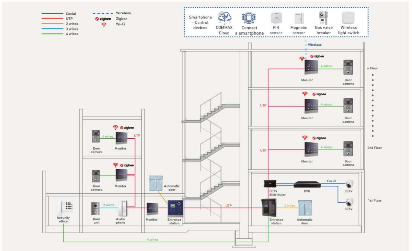
FIELD OF IoT GATE VIEW APPLICATION
