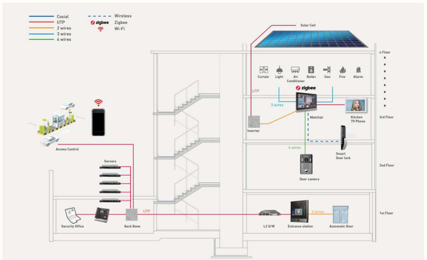
FIELD OF SMART HOME SYSTEM APPLICATION
