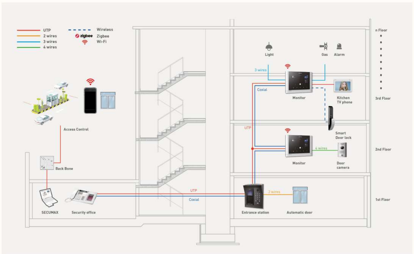
FIELD OF SMART GATE SYSTEM APPLICATION
