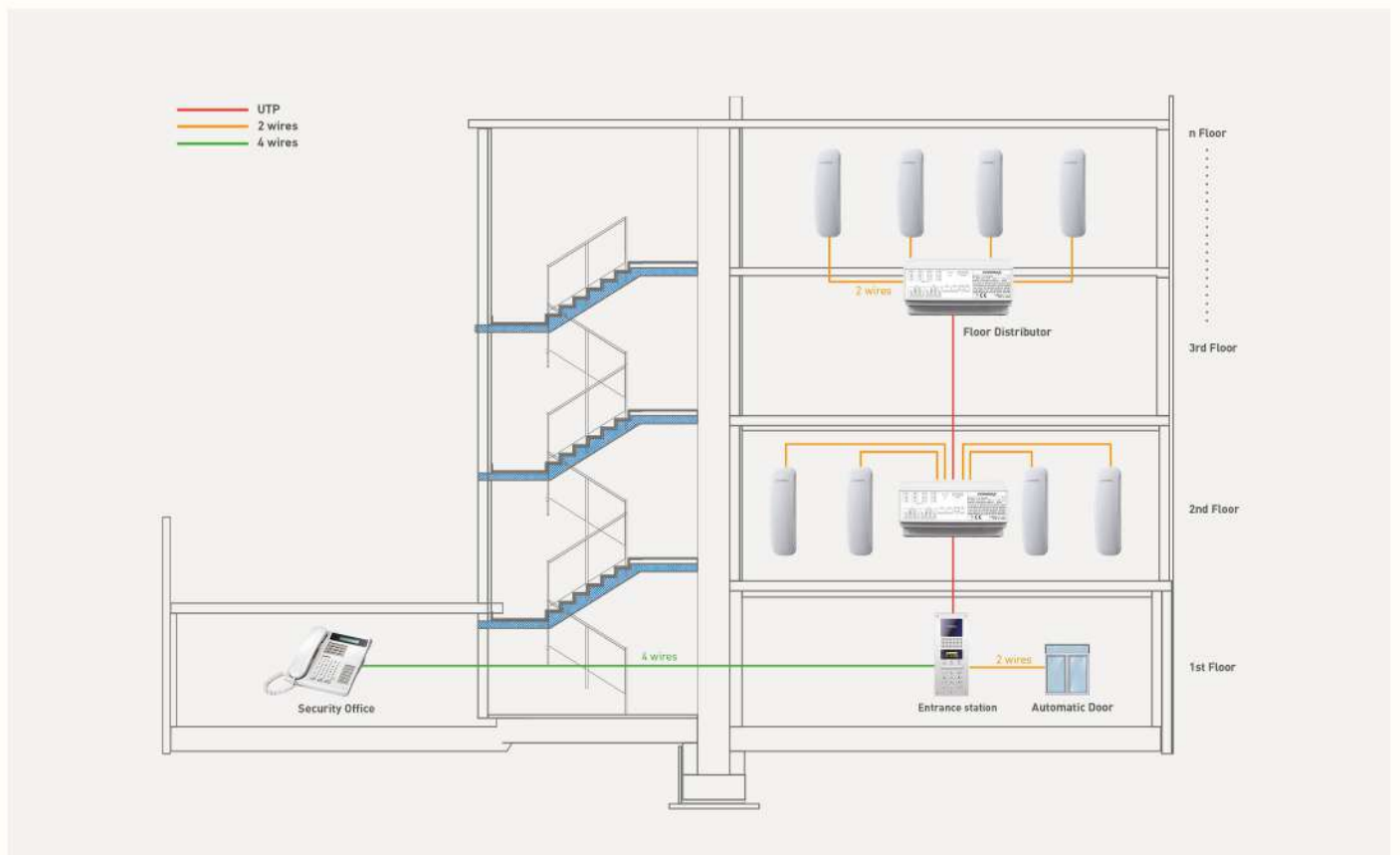
FIELD OF AUDIO GATE SYSTEM APPLICATION
